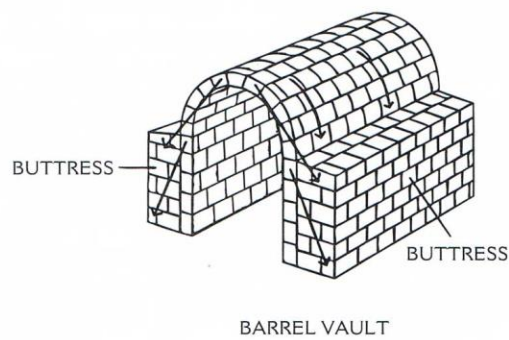
Figure 5.4 The arch, the barrel vault, and the groin vault.
